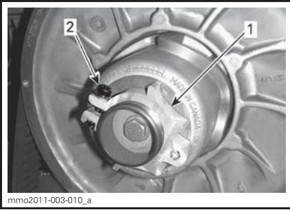
1. Adjuster hub 2. Clamping hub
