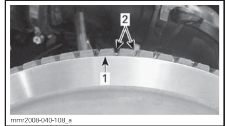
PRELIMINARY SETTING 1. Driven pulley edge 2. External drive belt grooves
