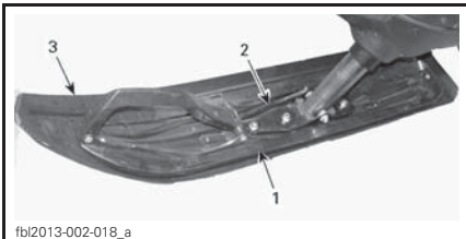
TYPICAL 1. Ski 2. Ski Runner 3. Ski Liner (Army model)
