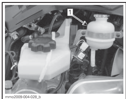
1. Coolant tank
