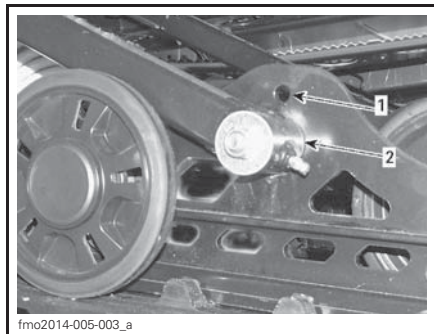
CENTER ARM 1. Position 1 2. Position 2
