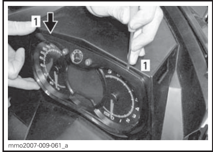
1. Locking tab
