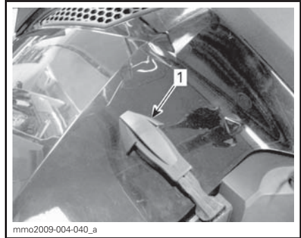
1. Rubber tie
