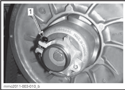
1. Clamping bolt
