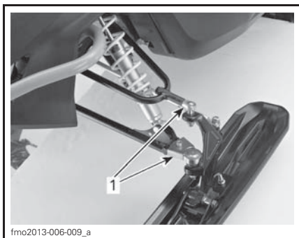
1. Widening kit
