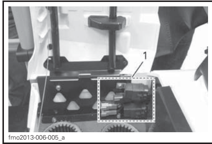
1. Accessory connections
