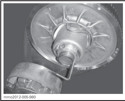
PULLEY EXPANDER ON ALUMINUM ADJUSTER HUB
