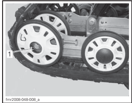
fmr2008-048-008_a 1. RH rear idler wheel bolt
