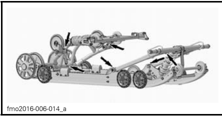
GREASE FITTINGS
