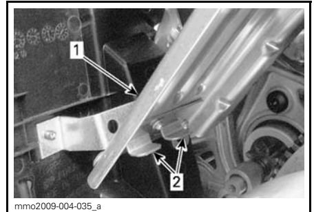
1. Drivreimvern 2. Tapper
