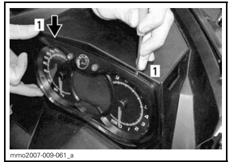
1. Locking tab
