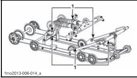
1. Grease fittings
