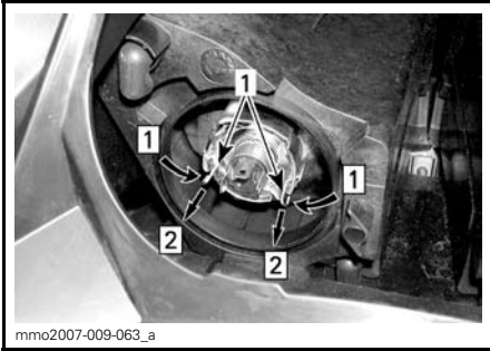
1. Retaining clip
