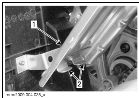
1. Drivreimvern 2. Tapper
