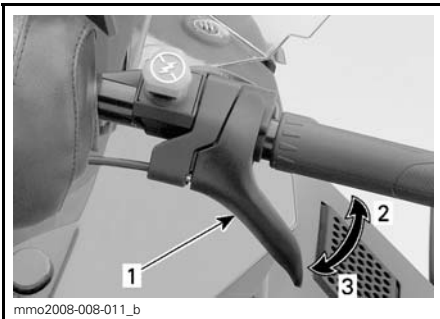
mmo2008-008-011_b TYPICAL 1. Throttle lever 2. To accelerate 3. To decelerate
