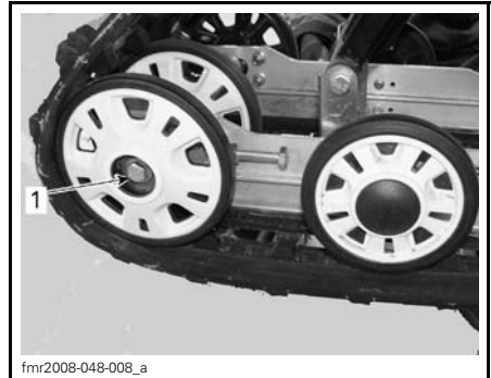
1. RH rear idler wheel bolt
