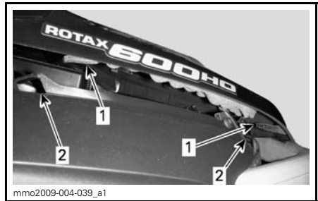
1. Tabs 2. Slots
