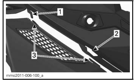
1. Console hook 2. Console slot 3. Panel center tabs
