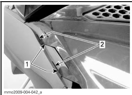
1. Tabs 2. Slots
