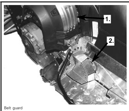
Belt guard
