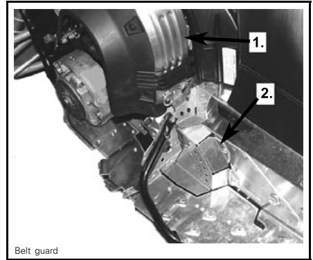
Belt guard
