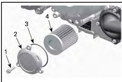
1. Oljefilterskruv
