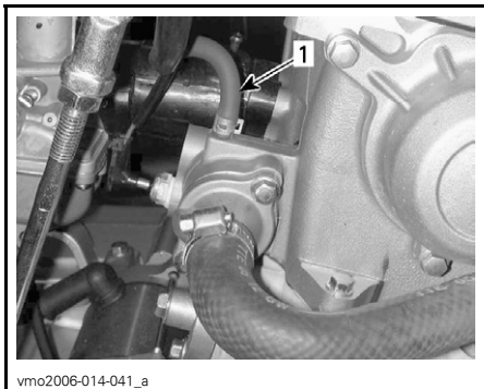
1. By-pass hose
