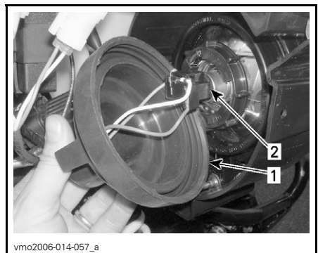
vmo2006-014-057_a 1. Remove rubber protector 2. Pull on connector using a wiggle movement
