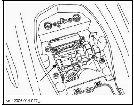
1. Fuse holder
