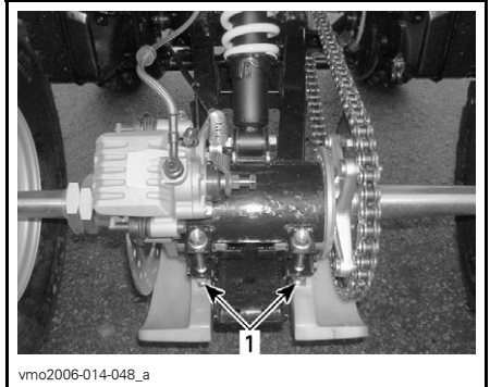
1. Chain tensioner lock bolts
