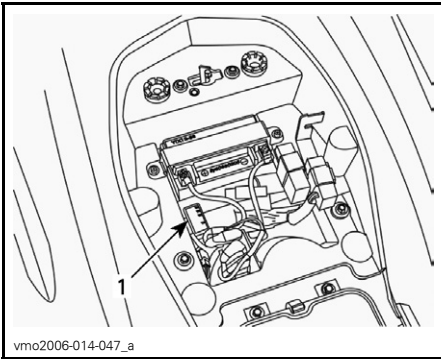
vmo2006-014-047_a 1. Fuse holder
