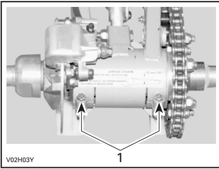
1. Rear axle lock bolts
