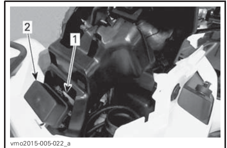
1. Front fuse box 2. Front fuse box cover
