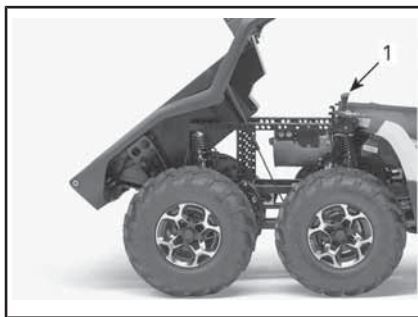
1. Hendel laadbed
