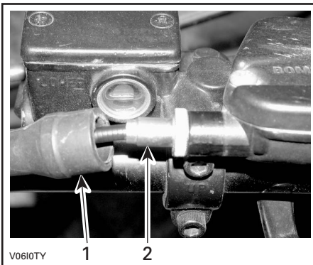
1. Rubber protector 2. Cable adjuster
