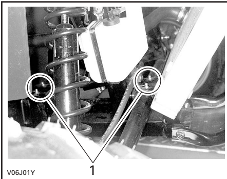
1. Grease fittings
