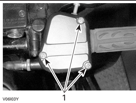
1. Remove screws
