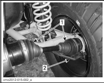
vmo2012-015-002_a TYPICAL — REAR OF VEHICLE 1. Drive shaft boots 2. Drive shaft protector
