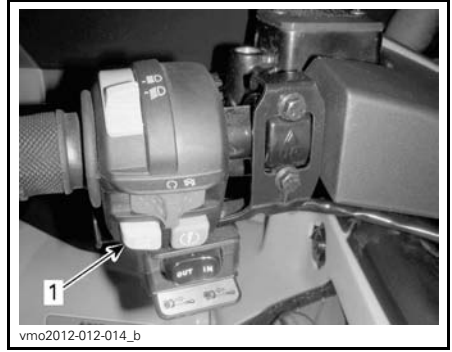
1. Override/DPS button
