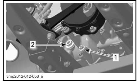
TYPICAL - 570/850 ENGINE
