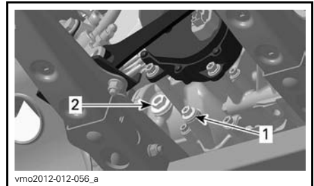
TYPICAL - 570/850 ENGINE
