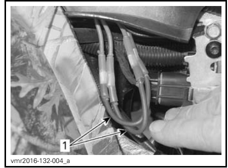
1. Fusible links
