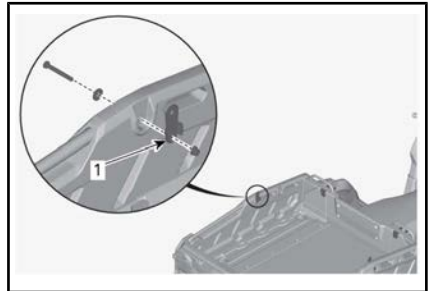
1. Staffe laterali
