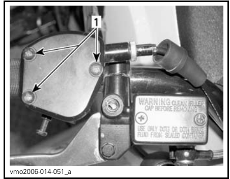
1. Remove screws
