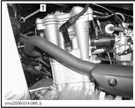
LH SIDE OF ENGINE 1. Air injection valve
