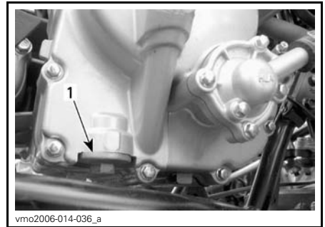
RH SIDE OF ENGINE
