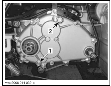
1. Gearbox drain plug 2. Gearbox fill plug
