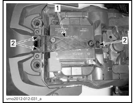
1. Battery holding strap 2. Retaining screws
