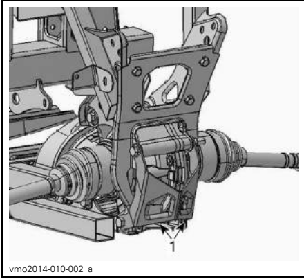
vmo2014-010-002_a 1. Recovery hook
