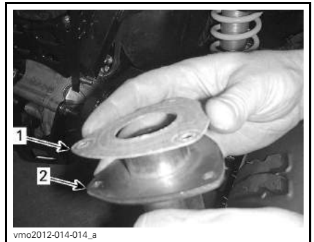
TYPICAL 1. Gasket 2. Exhaust tail pipe
