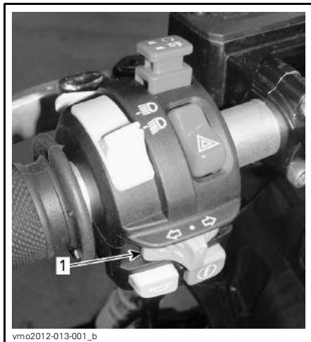
1. Turn signal switch
