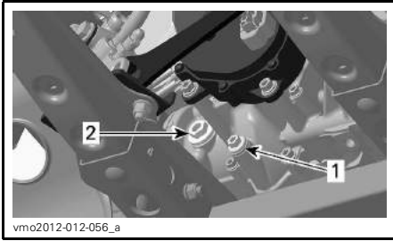
TYPICAL - 570/850 ENGINE
