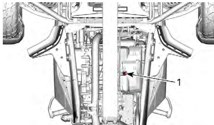
1. Dreneringsplugg for motorolje
