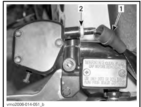
1. Rubber protector 2. Cable adjuster
