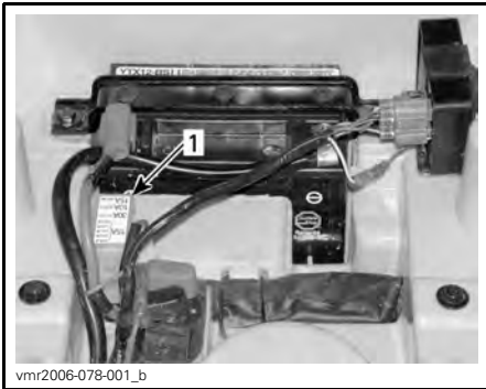
1. Fuse holder
