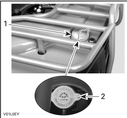
1. Radiator cap
