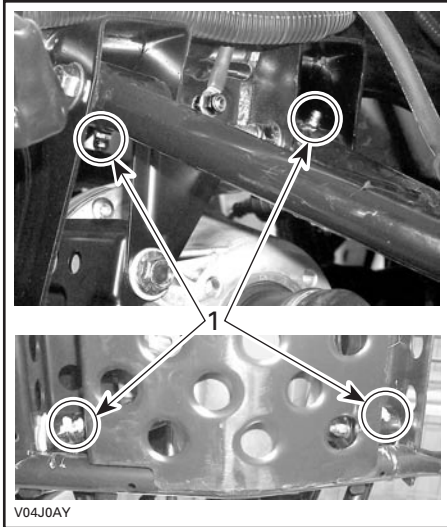
1. Grease fittings
