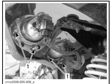
1. Adjustment screws
