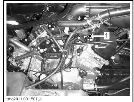
1. Front cylinder bleed screw
