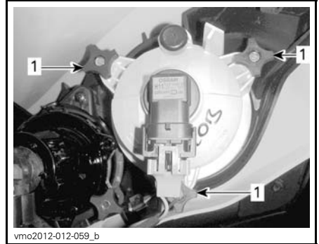
LOW BEAM ADJUSTMENT 1. Adjustment knobs
