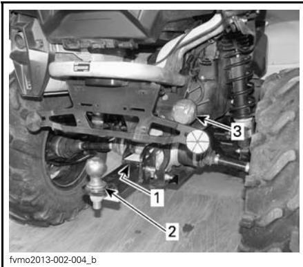
TYPICAL T3 MODEL 1. Towing instructions 2. Trailer Hitch 3. Trailer connector
