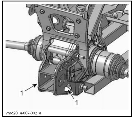
1. Recovery hook
