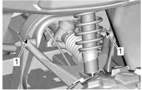
1. Smeefittingen ophangingsarm
