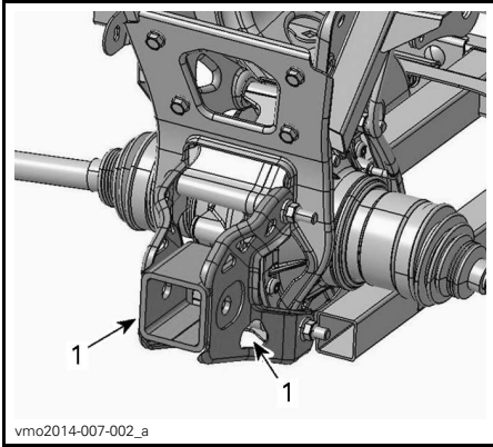
1. Recovery hook
