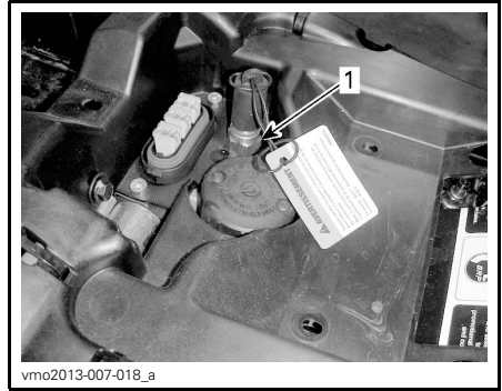
1. Compressor fitting
