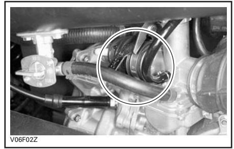
CHOKE LEVER IN THE FULL CHOKE POSITION
