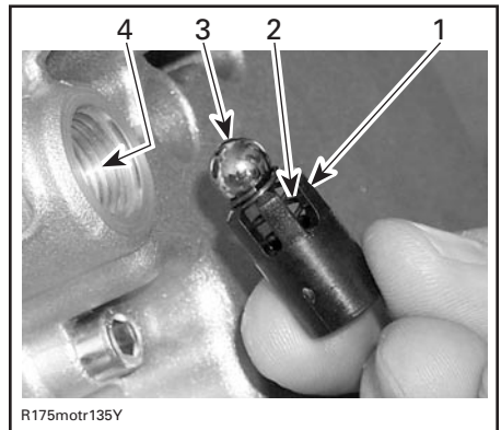
1. Valve housing 2. Compression spring 3. Ball 4. Oil pressure valve port
