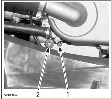
1. Cooling drain plug 2. Oil pressure regulator plug
