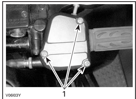
1. Remove screws
