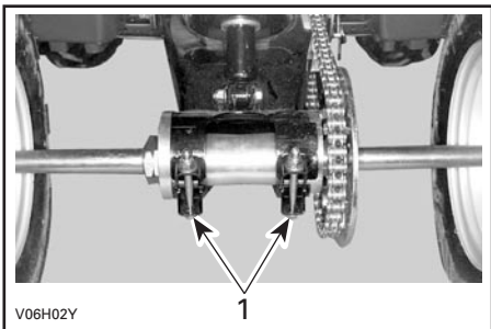
1. Chain tensioner lock bolts
