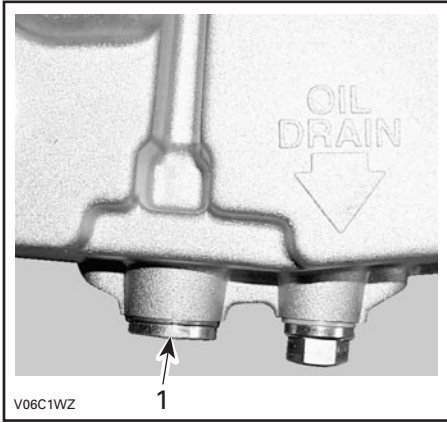
1. Oil strainer plug
