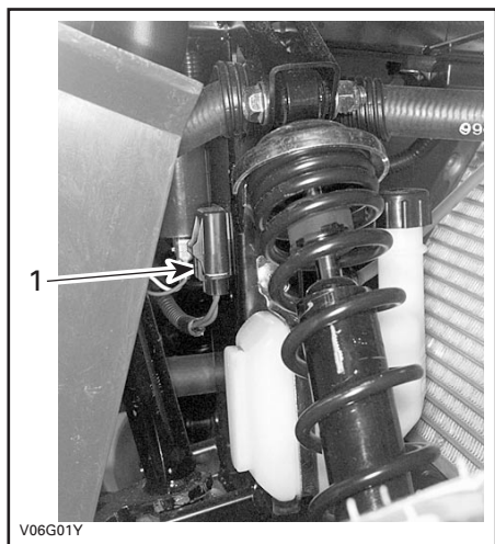
1. Fuse holder
