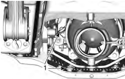
1. Opofferingsanodes
