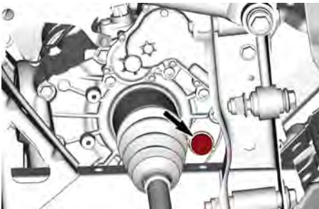
FRÄMRE SMART-LOK-DIFFERENTIAL
