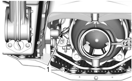
1. Sacrificial anodes
