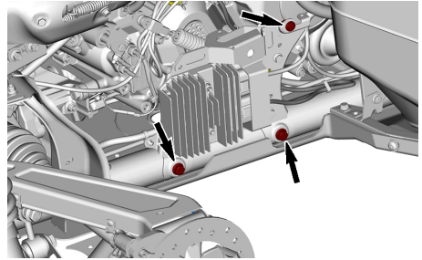
VOLTAGE/REGULATOR SUPPORT SCREWS
