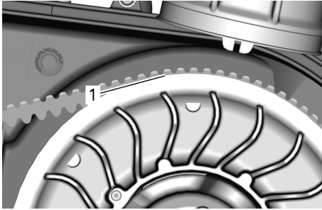
1. Lowest portion of cogs even with driven pulley edge
