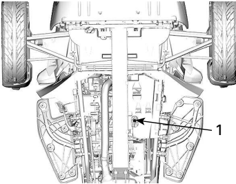
1. Engine oil drain plug
