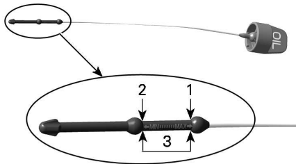
1. MAX 2. MIN 3. Operating range, 500 ml (17 fl oz(US))
