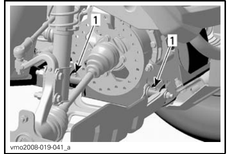
TYPICAL — RH SIDE 1. Grease fittings
