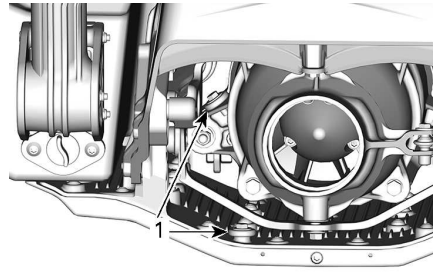
1. Sacrificial anodes
