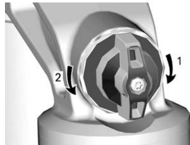
COMPRESSION DAMPING
