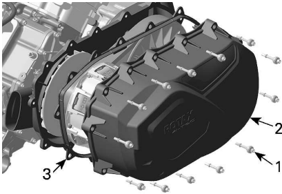
1. CVT cover screw 2. CVT cover 3. Gasket
