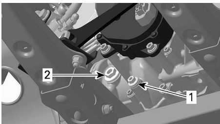
1. Drain plug 2. Oil level plug
