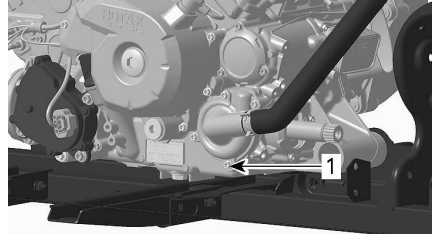
1. Coolant drain plug
