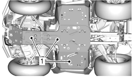
1. Protective plates
