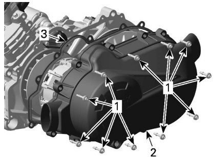
450 ENGINES 1. Retaining screws 2. CVT cover 3. Gasket
