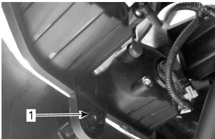
1. Adjustment screw
