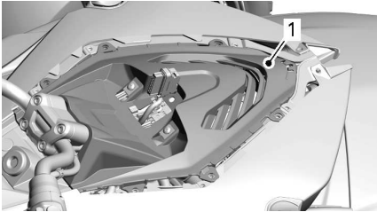
1. Console panel 11. Disconnect headlamp connector.
