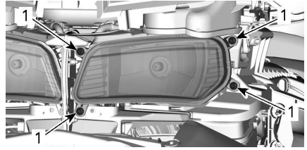
1. Headlight retaining screw 9. Disconnect headlamp connector.
