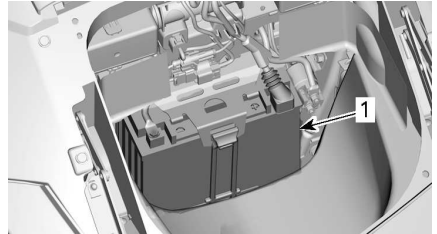
1. Battery
