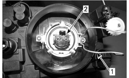
1. Bulb retaining spring 2. Bulb housing 14. Install the new bulb in place and secure with retaining spring.
