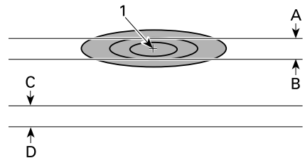
TYPICAL - HEADLIGHT REFLECTION ON TEST SURFACE — HIGH BEAM (SINGLE HEADLAMP)
