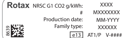
TYPICAL - NRMM IDENTIFICATION LABEL
