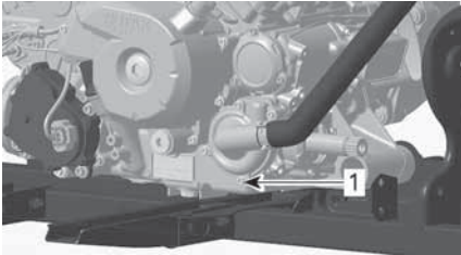
1. Coolant drain plug 650 Engines
