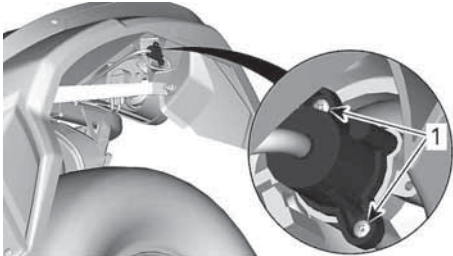
1. Rear turn signal light screws 2. Replace the light bulb. 3. Reinstall the socket.
